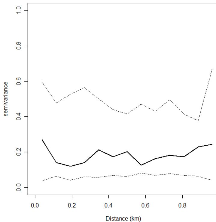
Figure 2.8 Omnidirectional semivariogram fitted to farm frailty for mortality on smallholder dairy farms in Tanga and Iringa regions of Tanzania during 1998
